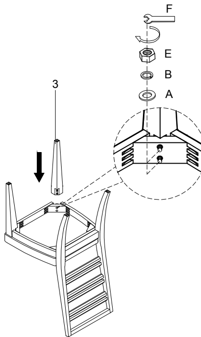
255927/D5100-62 Centre Side Chair
