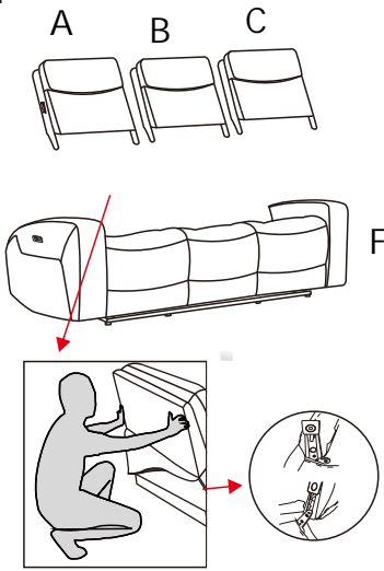
Fix the backrest by metal lock
